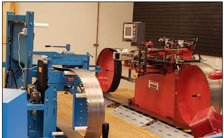
Left Image - Manual Bench. #81 Bench with welding clamp and #5 Super Duty Stretcher Roll. Right Image - Automated Bench. 095 AB with dual tension rolls and light curtain shutoff.
